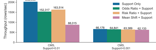
Figure 8: Throughput of different difference metrics on CMS, with a fixed ratio of 2.0 (except for Support Only).
